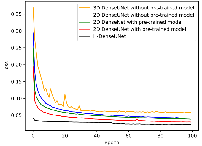
Fig. 3. Training losses of 2D DenseUNet with and without pre-trained model, 2D DenseNet with pre-trained model, 3D DenseUNet without pre-trained model as well as H-DenseUNet (Best viewed in color).
